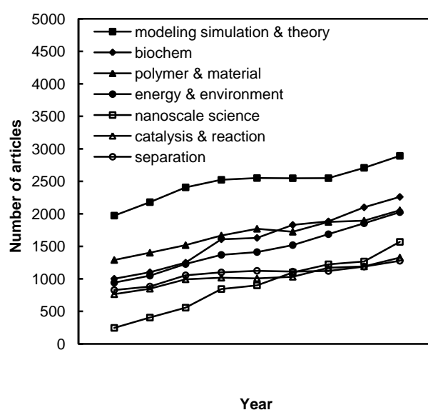
Figure 2. Comparison of the growth trends of seven research areas related to CE.
