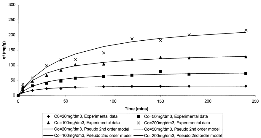
Figure 6. Plot of sorbed amount versus time for Astrazon Blue (BB69) at various initial concentrations.
