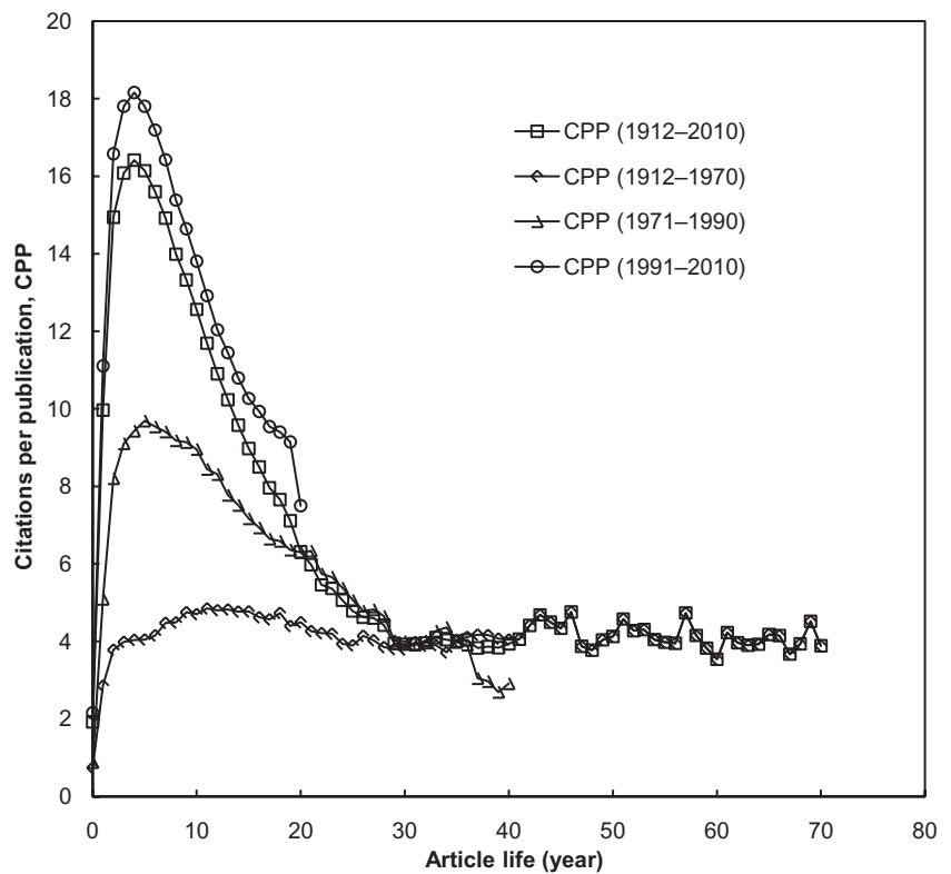
Figure 2 Variations of citations per article with article life.
