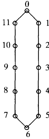
FIG. 16. Labeling of points in "worm" shapes.
