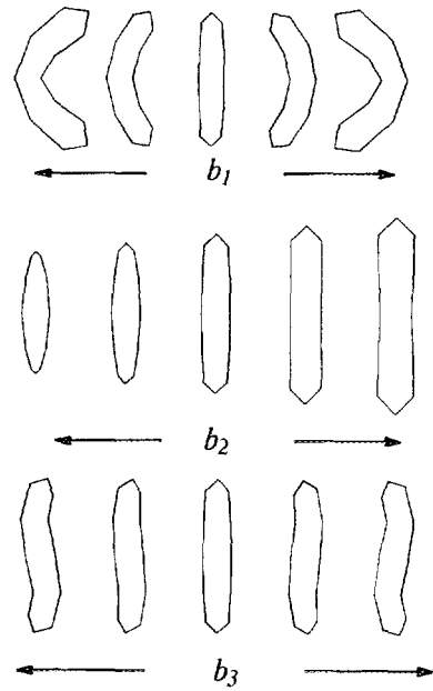
FIG. 18. Effects of varying the first three parameters ( b_1 , b_2 , b_3 ) of the "worm" model individually.
