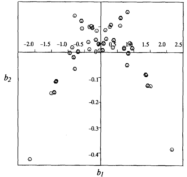
FIG. 19. b_1 vs b_2 for the training set of "worm" examples.
