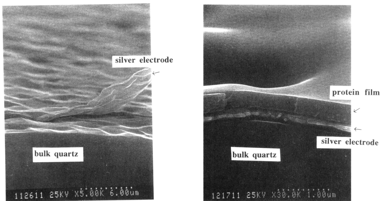
Figure 1. Scanning electron micrographs: (left) silver electrode deposited onto the quartz resonator (part of the silver layer is detached from the quartz); (right) {(PEI/PSS) 2 + (PEI/GOD) 8 + PEI} film deposited onto the silver-coated resonator.
